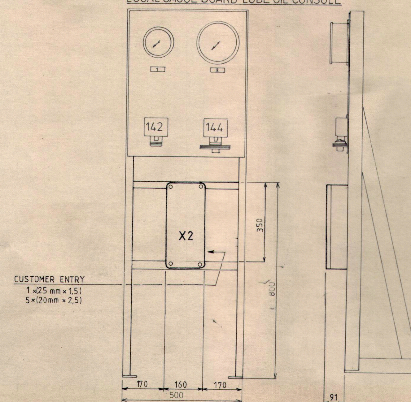
LOCAL GAUGE BOARD LUBE OIL CONSOLE
