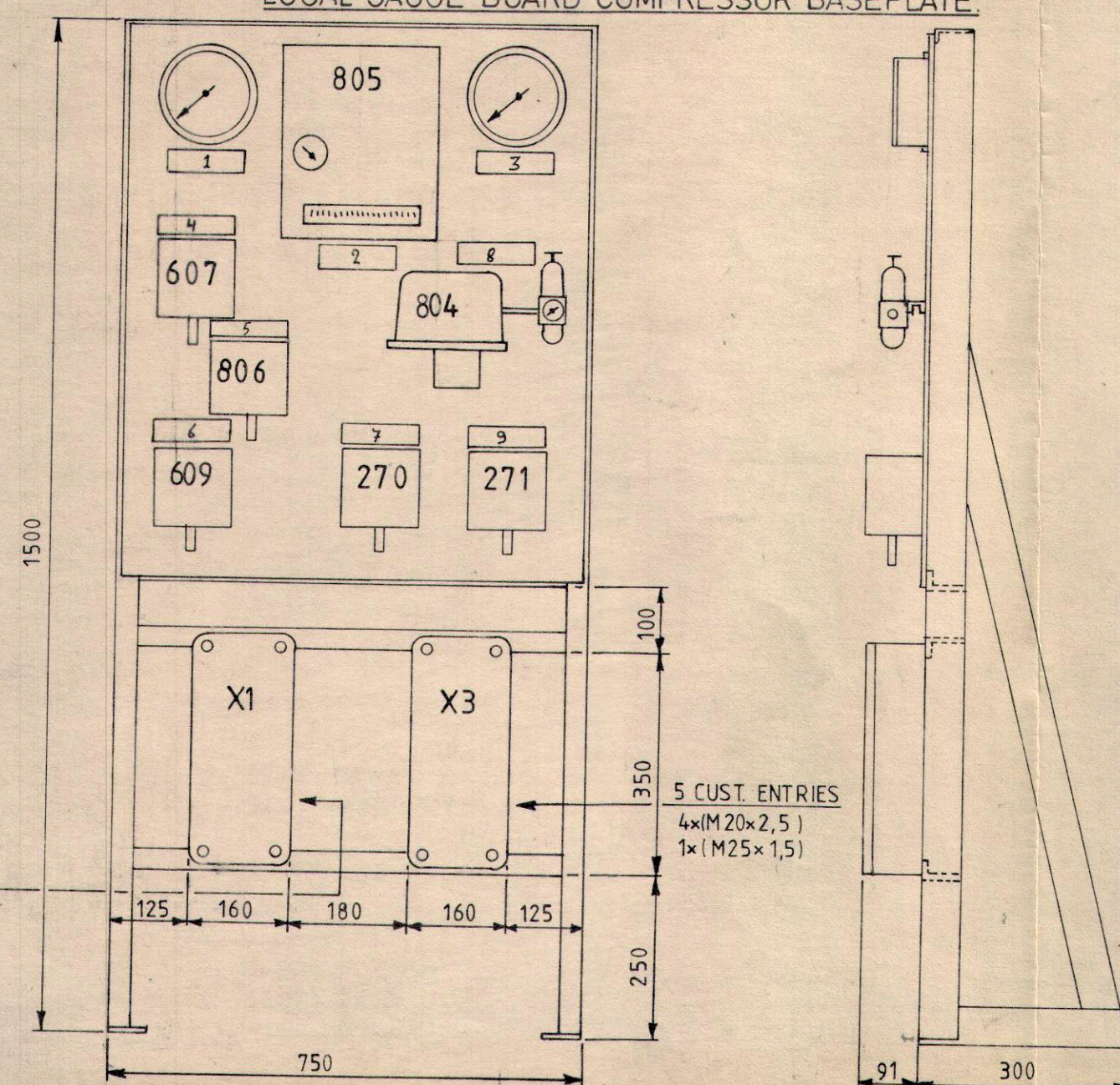
LOCAL GAUGE BOARD COMPRESSOR BASEPLATE
