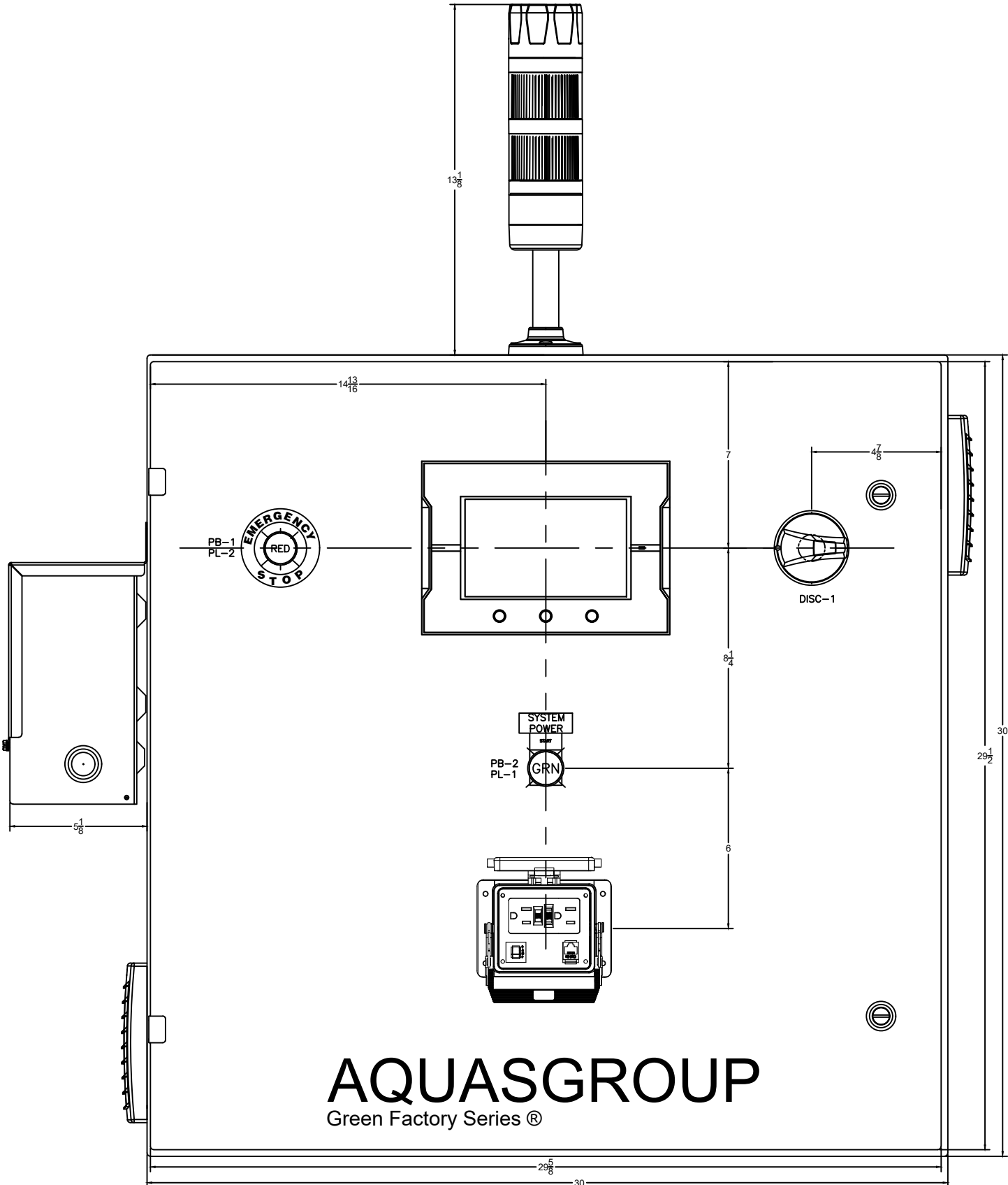
FRONT VIEW
