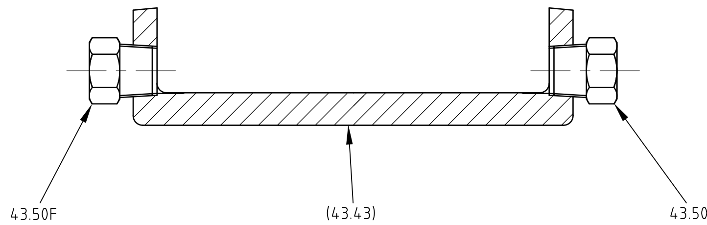
SCRAP VIEW OF COUPLING HOUSING VIEW ON ARROW A
