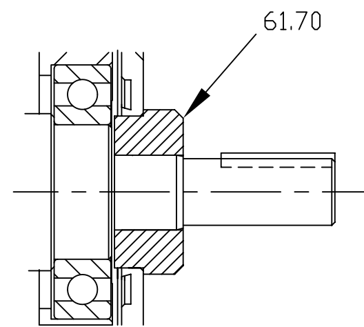
BEARING HOUSING FITTED WITH IMPRO SEAL
