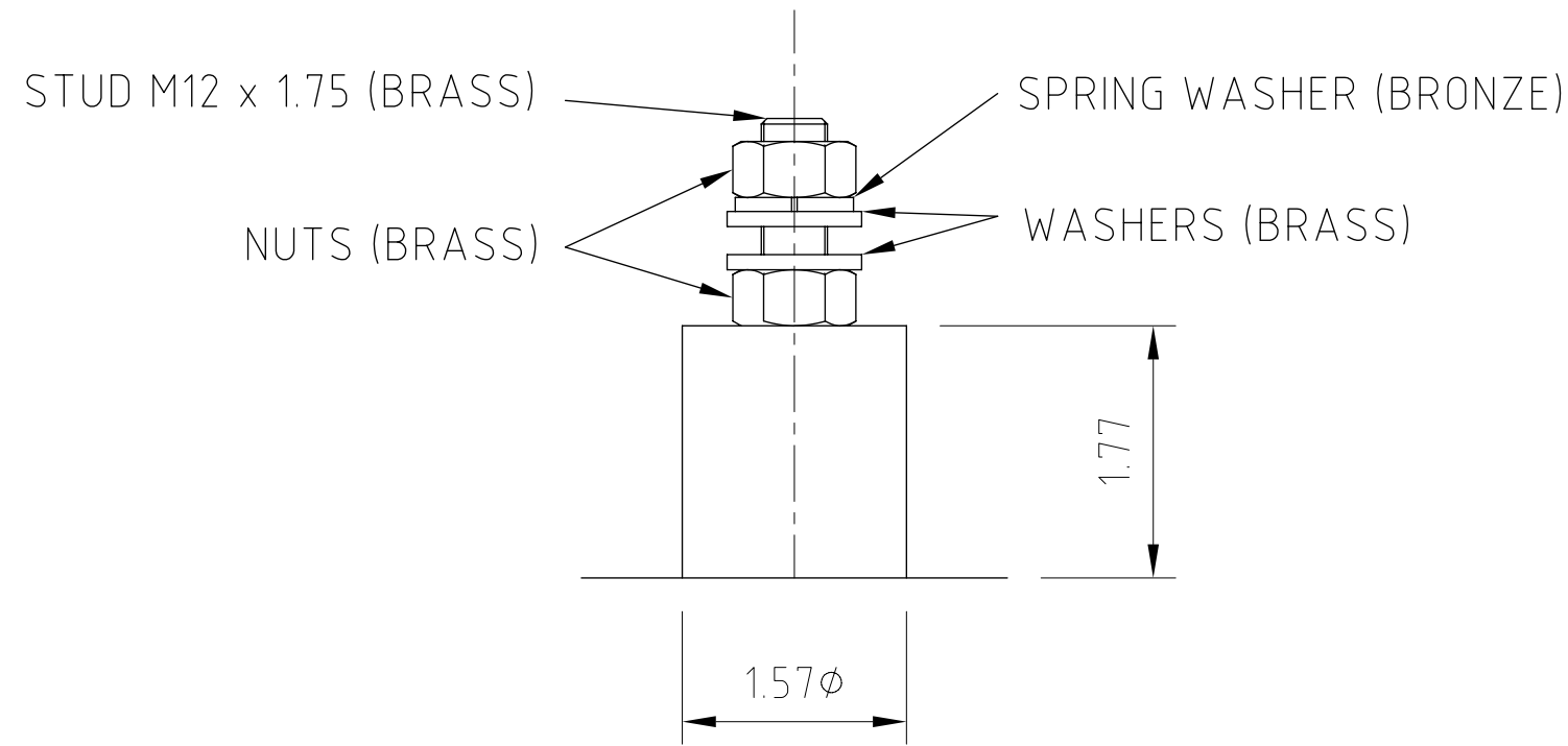
EARTHING BOSS DETAIL SCALE 1:2
