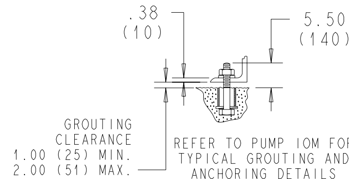
TYPICAL ANCHOR BOLT INSTALLATION
