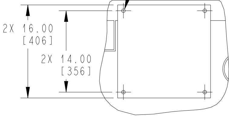
DETAIL D SCALE 1:10
