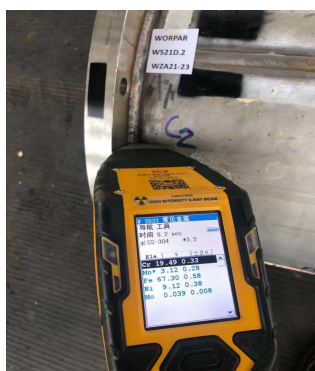
WELD C2
