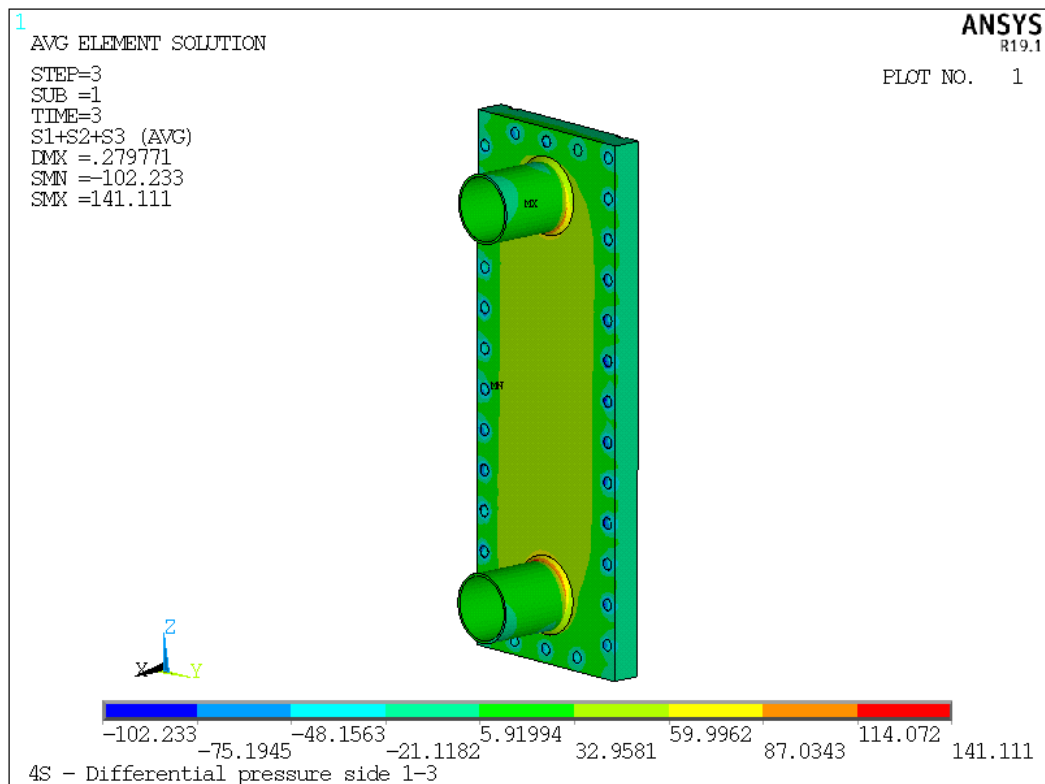
Figure 22: Sum of Principal stresses S1 + S2 + S3 - differential pressure side A
