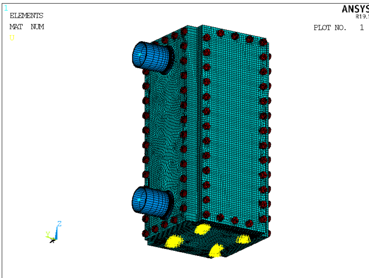
Figure 8: Boundary conditions
