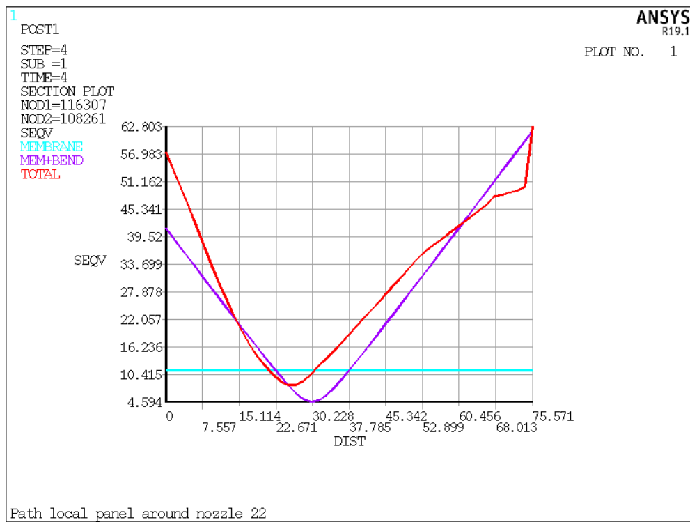
Figure 51: Maximal local path of the panel 2 around the nozzle 2
