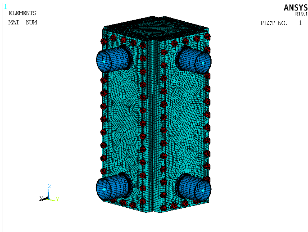
Figure 3: meshing
