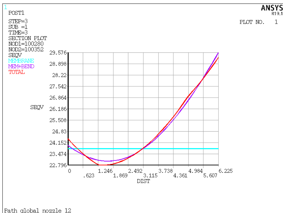
Figure 42: Maximal path of the global zone for the nozzle 2
