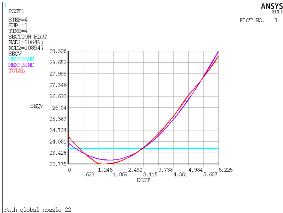
Figure 52: Maximal path of the global zone for the nozzle 2
