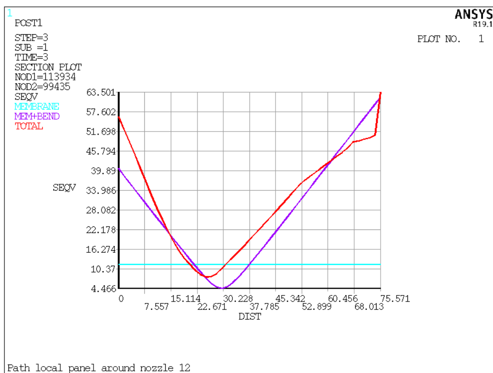
Figure 41: Maximal local path of the panel 1 around the nozzle 2
