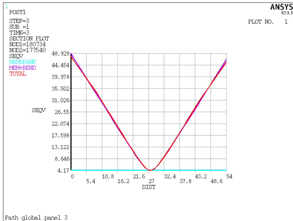
Figure 44: Maximal path of the global zone for the panel 3
