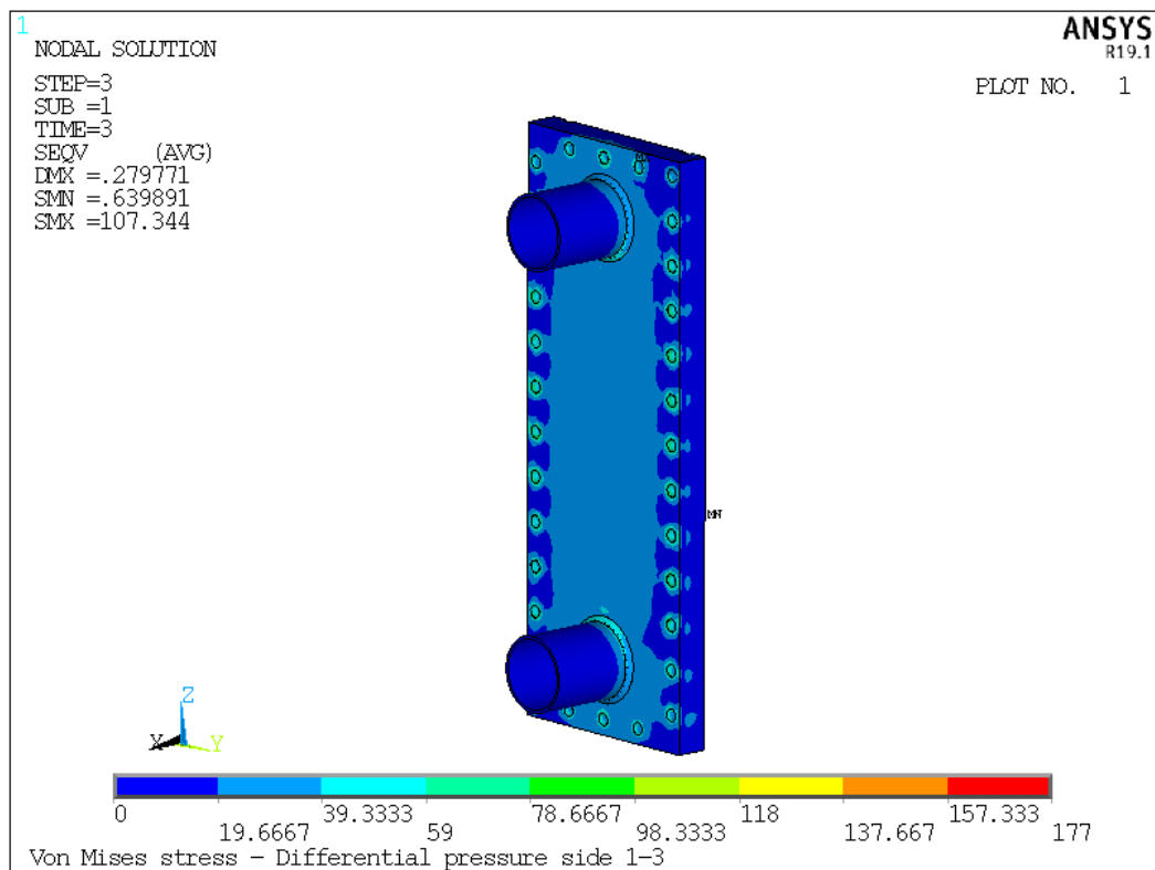
Figure 21: Von Mises stress - differential pressure side A
