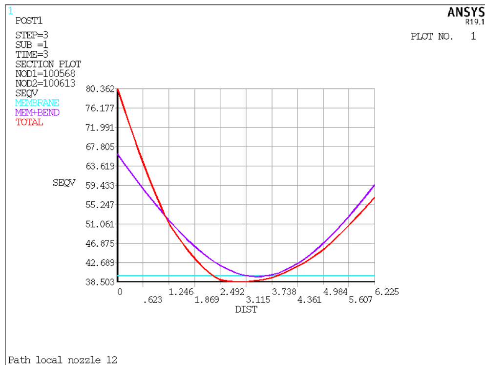
Figure 43: Maximal path of the local zone for the nozzle 2
