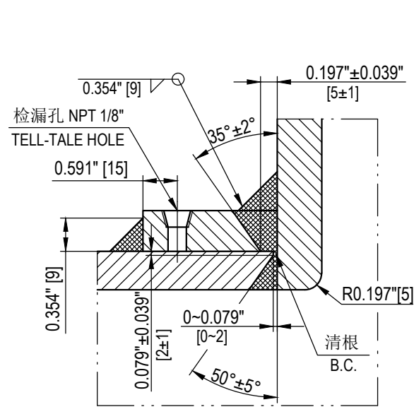
"W2"焊缝详图 DETAIL OF "W2" WELD
