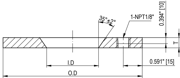
补强圈详图 DETAIL OF REINFORCEMENT PAD
