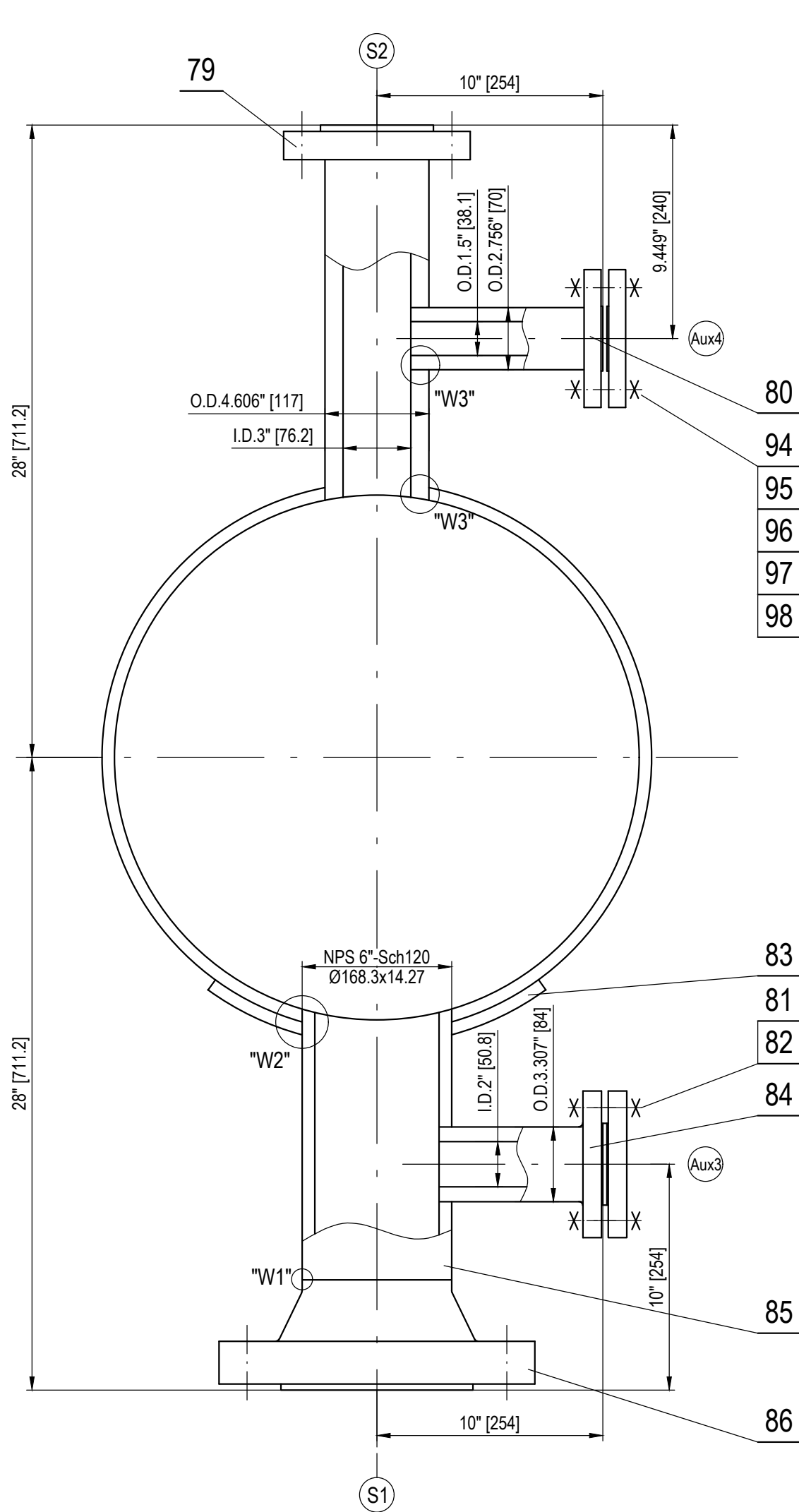
接管S1,S2,Aux3,Aux4详图 DETAIL OF NOZZLE S1,S2,Aux3,Aux4
