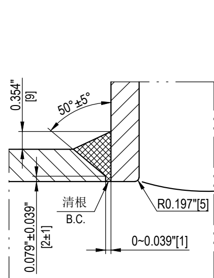
"W3"焊缝详图 DETAIL OF "W3" WELD
