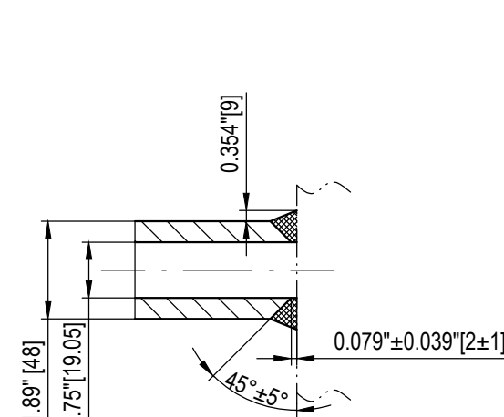
"W4"焊缝详图 DETAIL OF "W4" WELD
