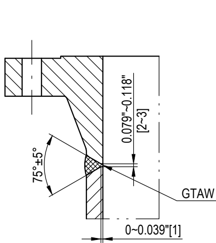
"W1"焊缝详图 DETAIL OF "W1" WELD
