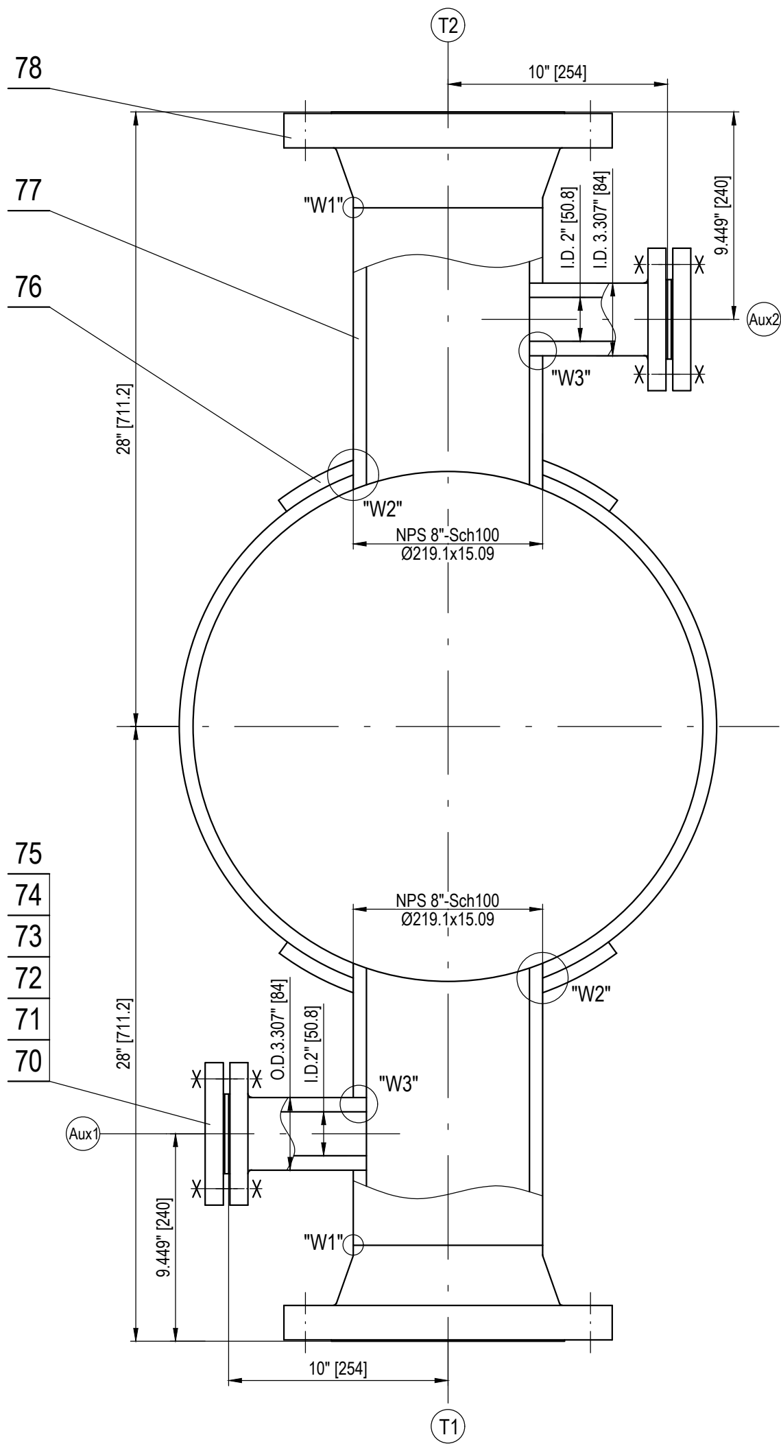
接管T1,T2,Aux1,Aux2详图 DETAIL OF NOZZLE T1,T2,Aux1,Aux2
