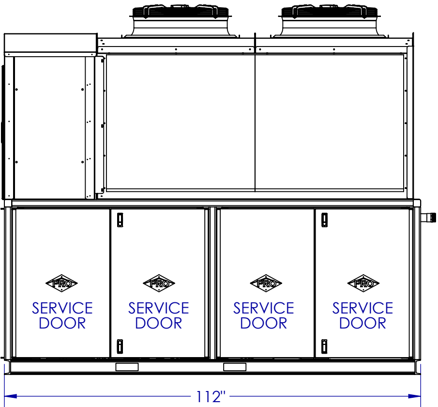
SIDE VIEW
