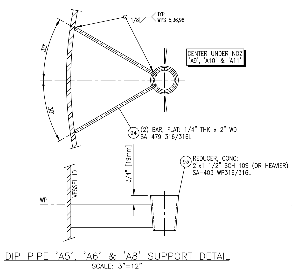
DIP PIPE 'A5', 'A6' & 'A8' DETAIL SCALE: 3"=12"
