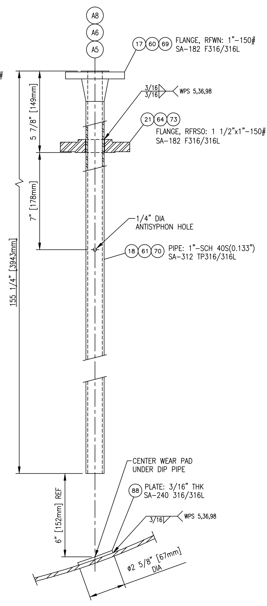
DIP PIPE 'A5', 'A6' & 'A8' DETAIL SCALE: 3"=12"
