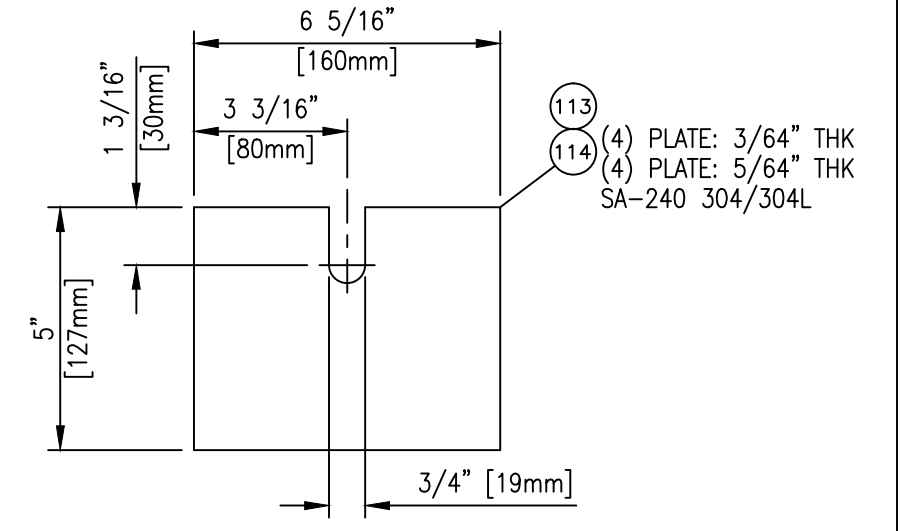
ADJUSTING PLATE DETAIL TYP (8) PLACES (SHIP LOOSE) SCALE: 3"=12"
