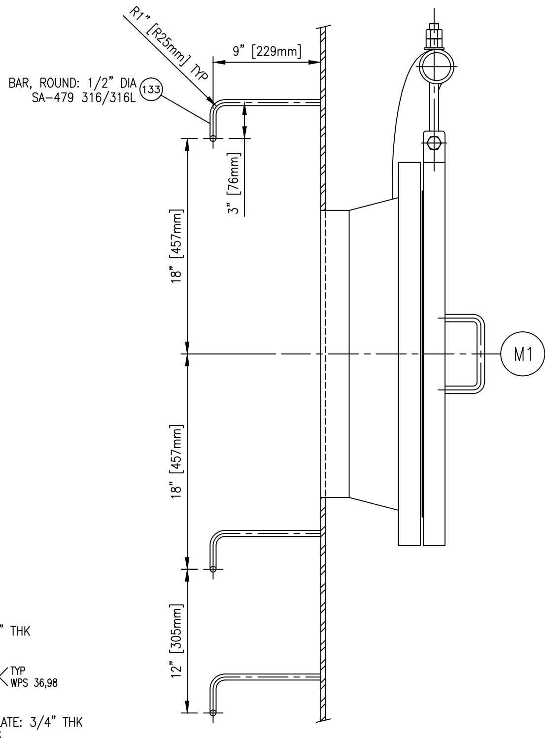
INTERNAL GRAB RUNG DETAIL SCALE: 1 1/2"=12"
