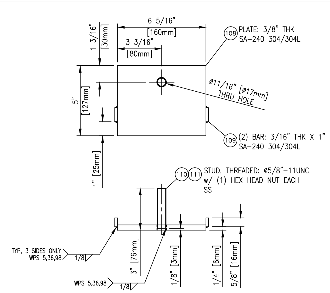
WELD PLATE DETAIL TYP (4) PLACES (SHIP LOOSE) SCALE: 3"=12"
