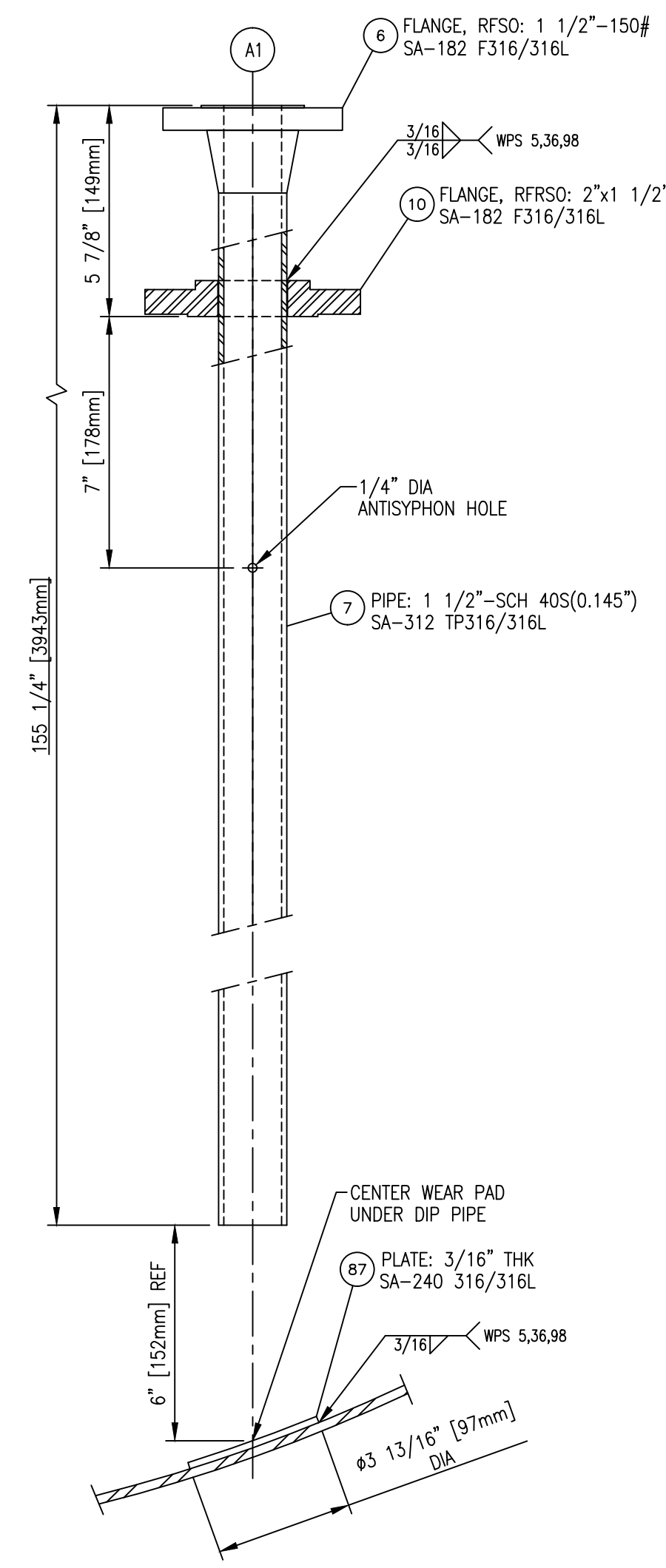
DIP PIPE 'A1' DETAIL SCALE: 3"=12"
