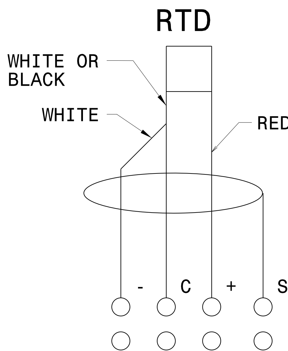
TYPICAL BEARING TEMPERATURE DETECTOR
