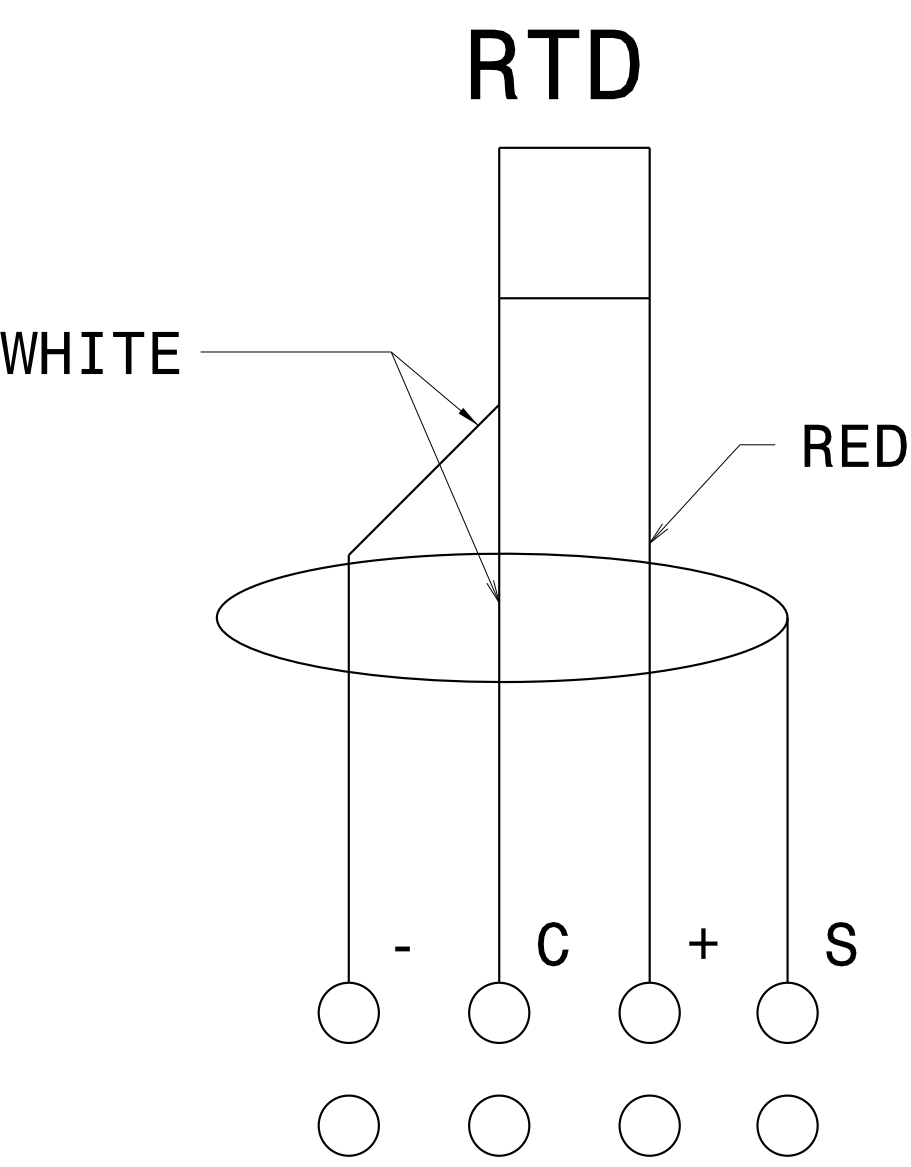
TYPICAL STATOR TEMPERATURE DETECTOR
