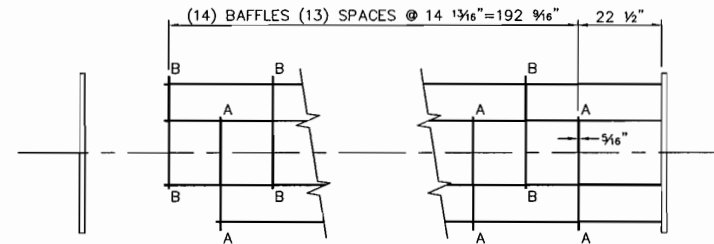
BUNDLE DETAIL
