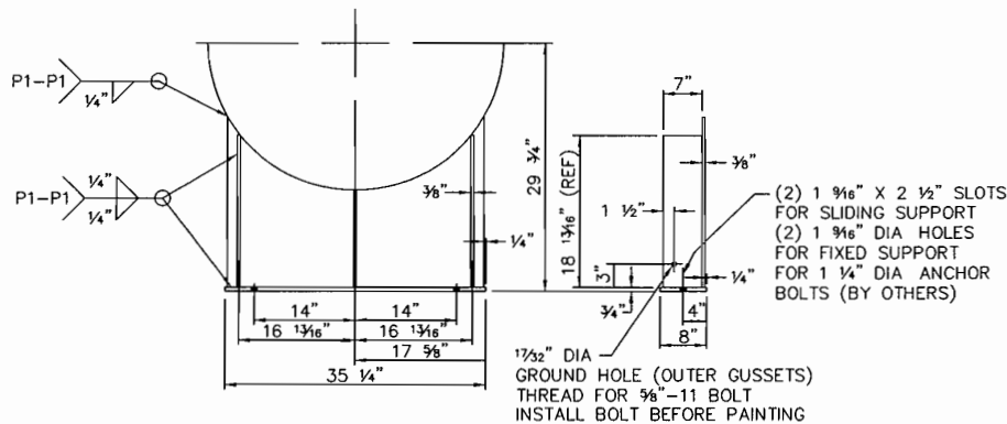
SUPPORT DETAIL
