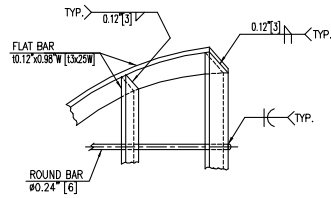
DETAIL OF GRID
