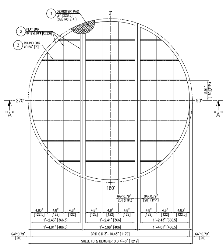
PLAN VIEW OF DEMISTER
