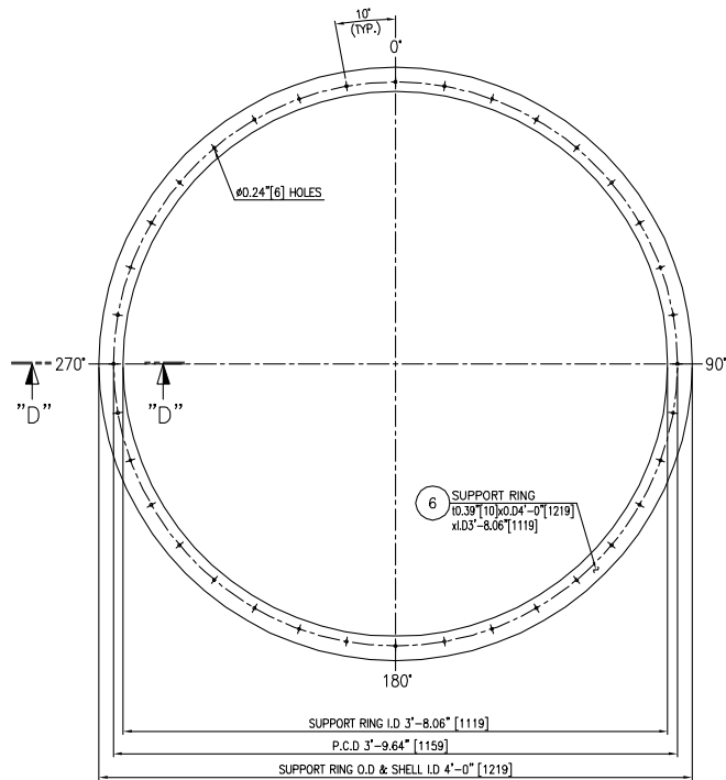
PLAN VIEW OF SUPPORT RING
