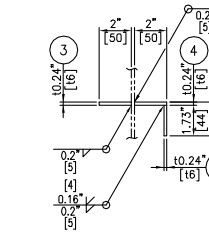
SECTION "F"
