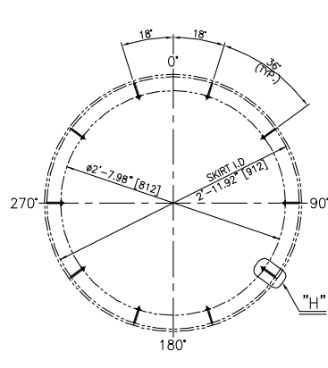
VIEW "D"
