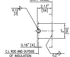
DETAIL "G"
