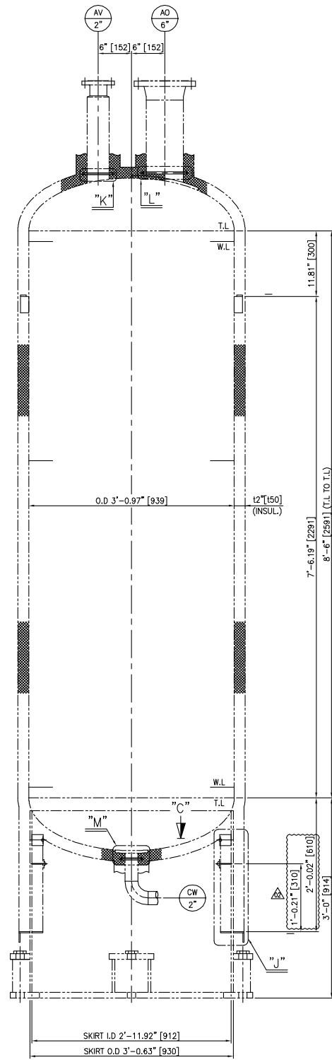
ELEVATION VIEW
