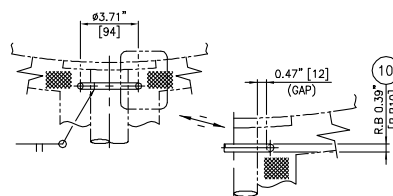
DETAIL "M"
