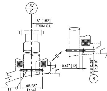
DETAIL "K"
