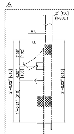
DETAIL "J"
