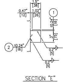
SECTION "E"
