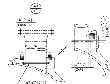
DETAIL "L"
