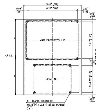
DETAIL OF BRACKET
