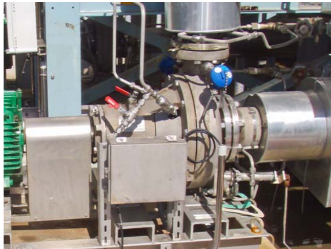
Wilfley pump with thermowells and crust breaker valve
