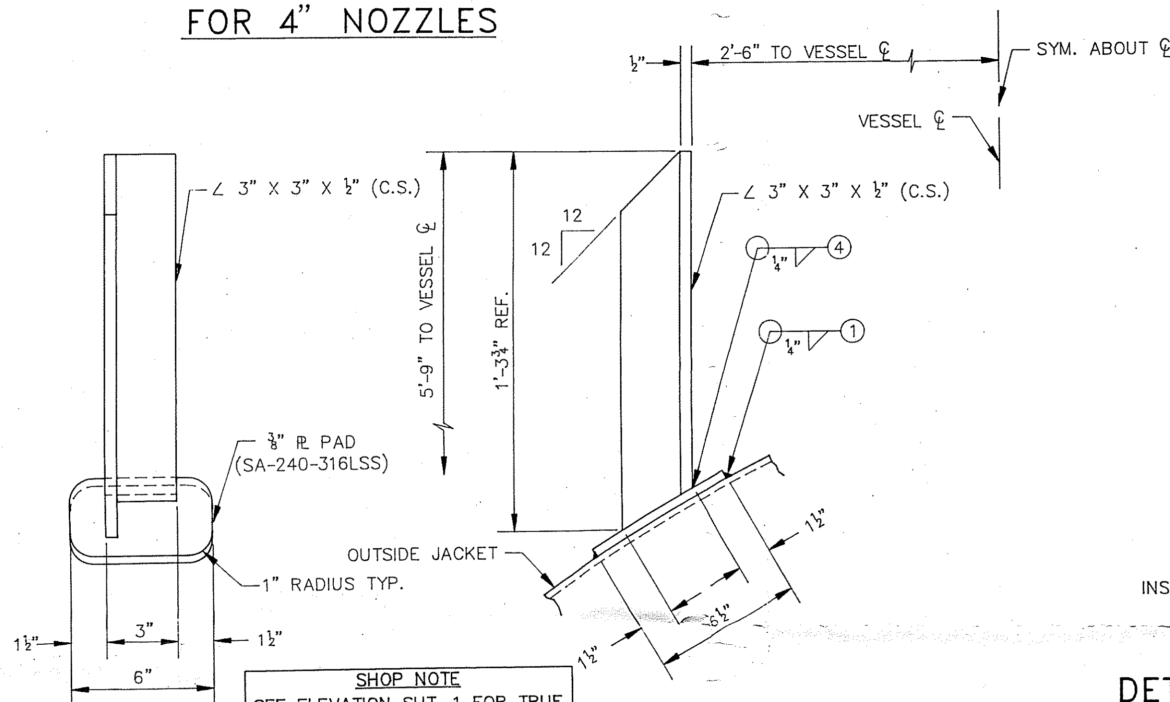
DETAIL OF WALKWAY CLIPS (8) REQ'D.
