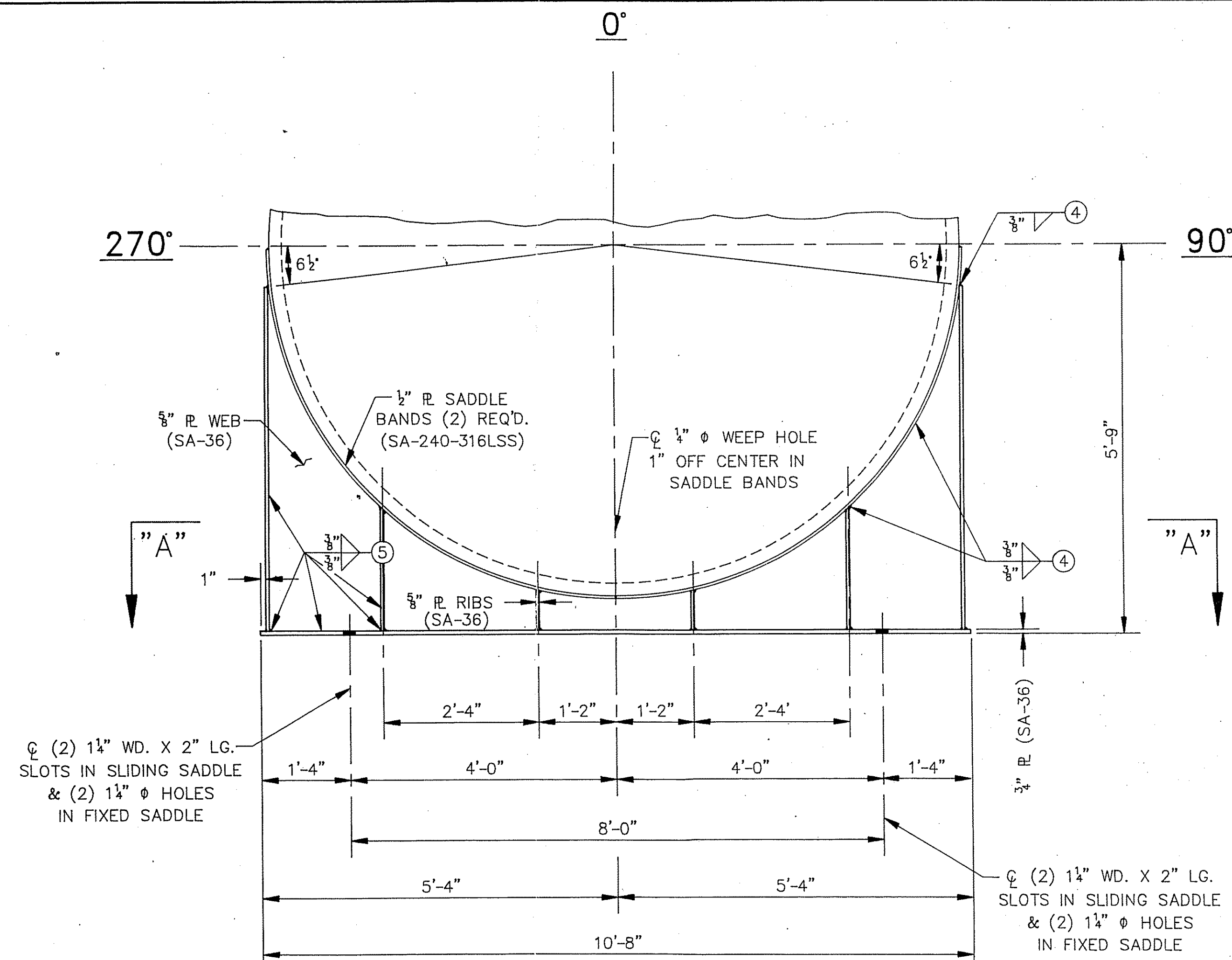
DETAIL OF SADDLES (2) REQ'D.
