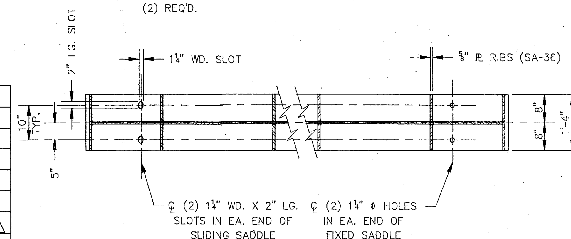
VIEW "A"
