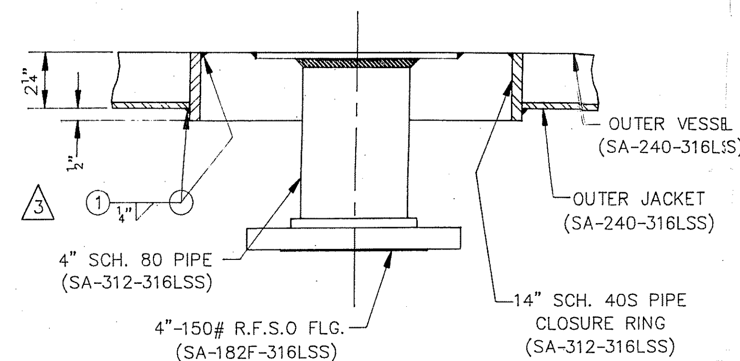
TYP. CLOSURE BAR DETAIL FOR 4" NOZZLES
