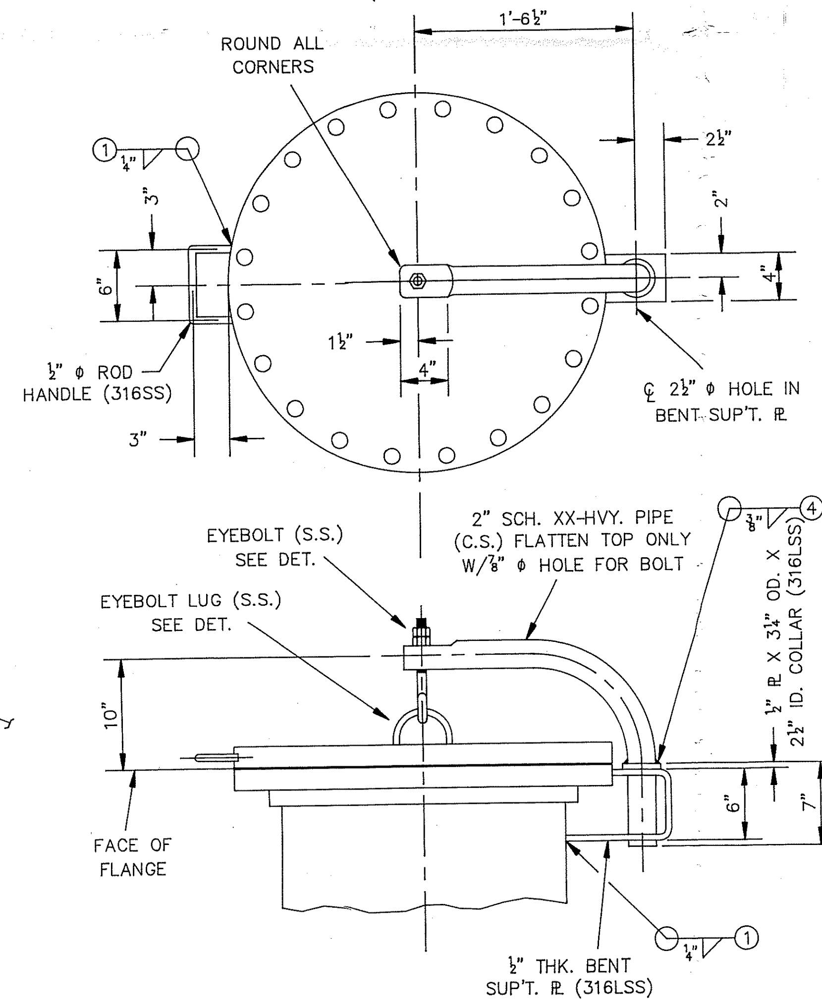
DETAIL OF DAVIT @ MANWAY "MW" (1) REQ'D
