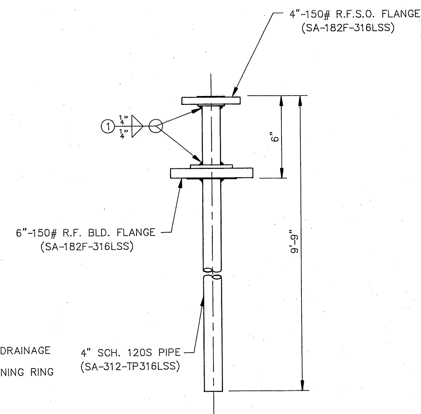
DETAIL OF DIP PIPE @ NOZZLE "B" (1) REQ'D
