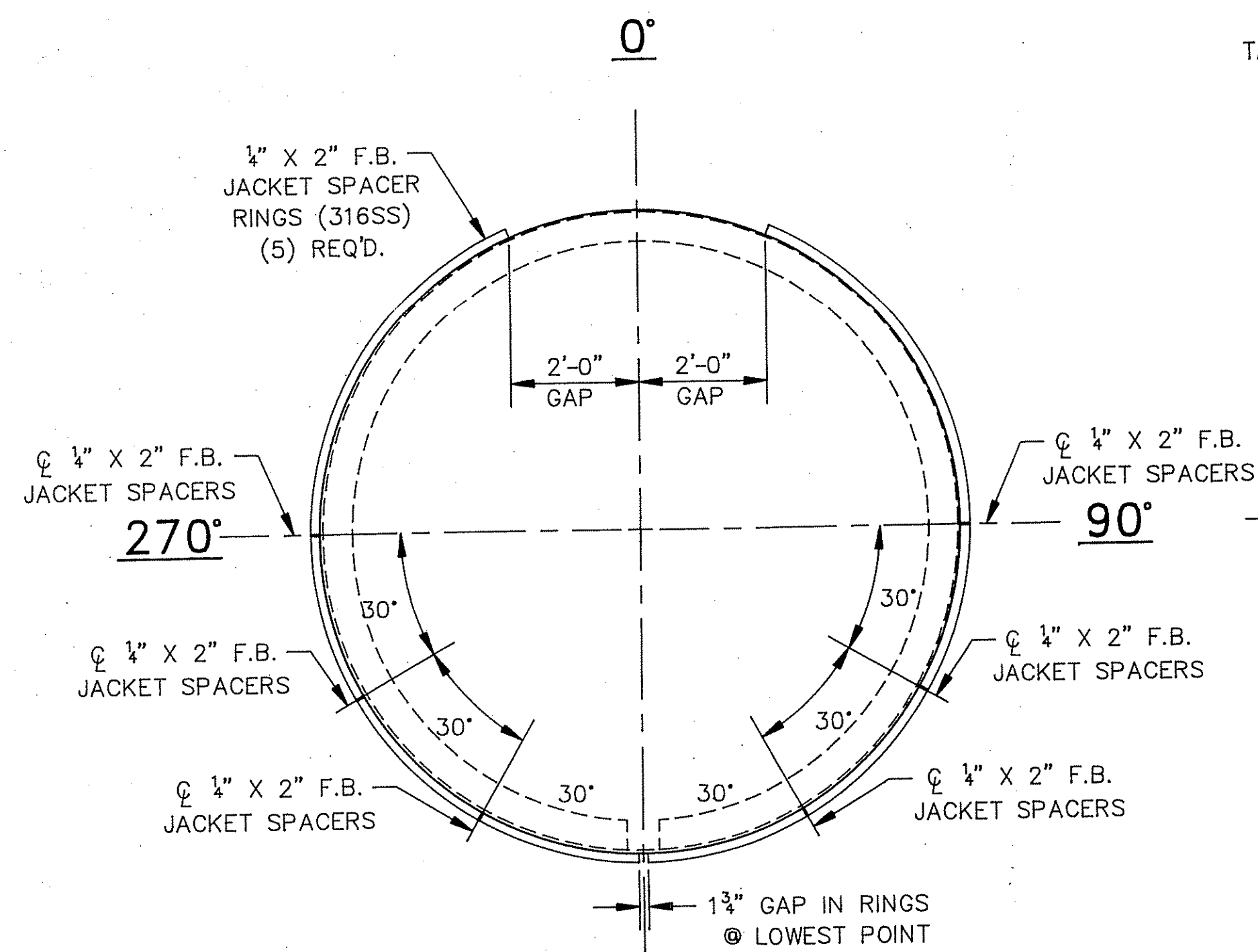
180° END VIEW
