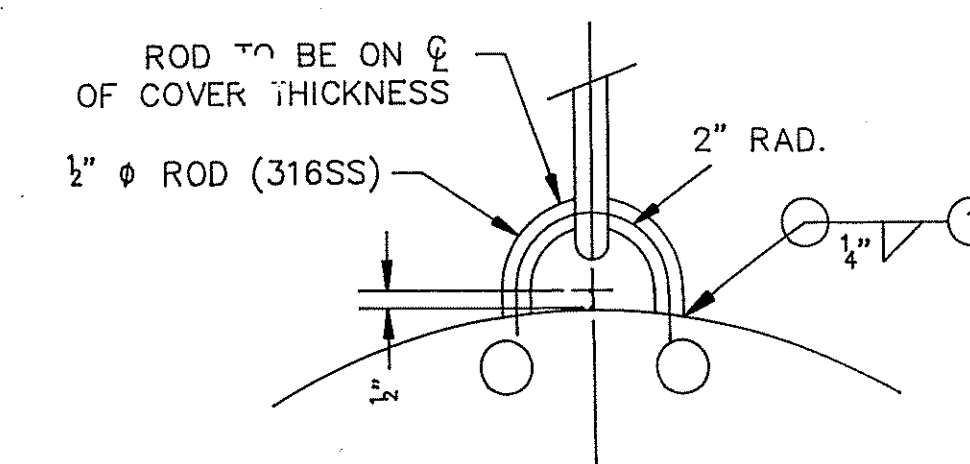
DETAIL @ EYEBOLT LUG (1) REQ'D
