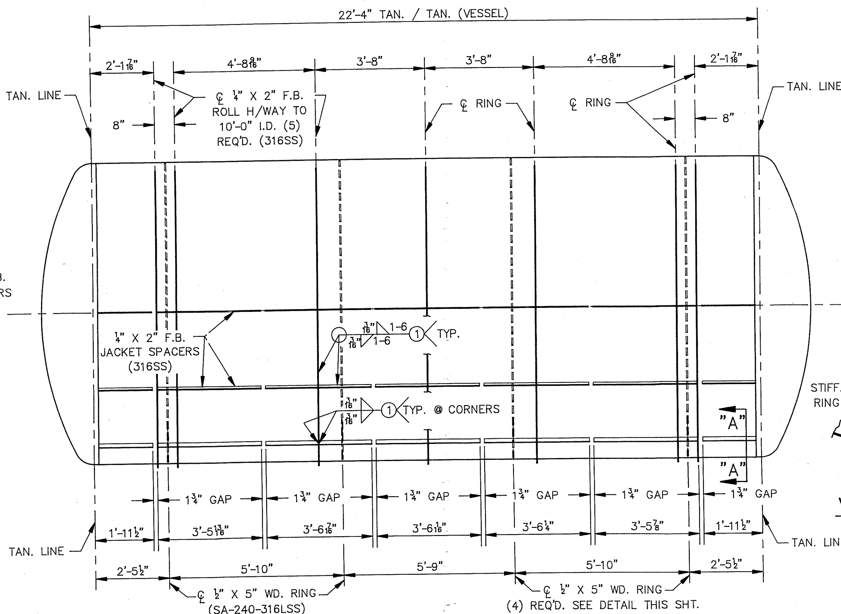
DETAIL OF JACKET SPACERS & INT. STIFF. RINGS (VESSEL SHOWN WITHOUT JACKET FOR THE SAKE OF CLARITY)
