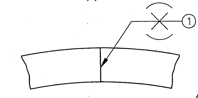
DETAIL OF TYP. RING SPLICE
