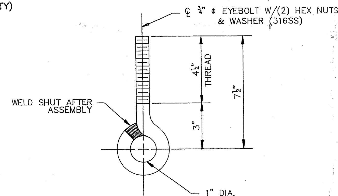
DETAIL @ EYEBOLT (1) REQ'D
