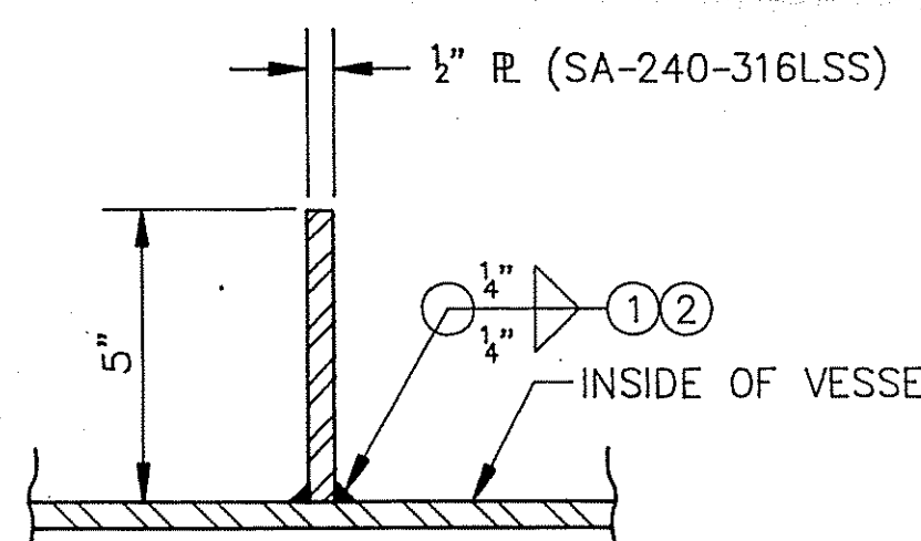
DETAIL OF STIFFENING RINGS (4) REQ'D
