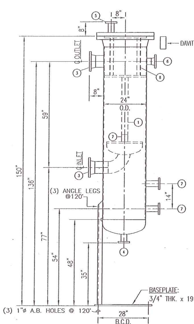
ELEVATION VIEW
