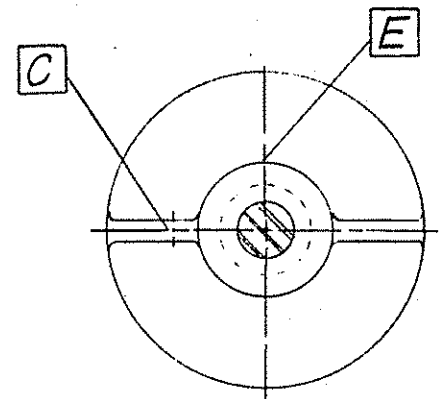
VIEW "X"-X"
