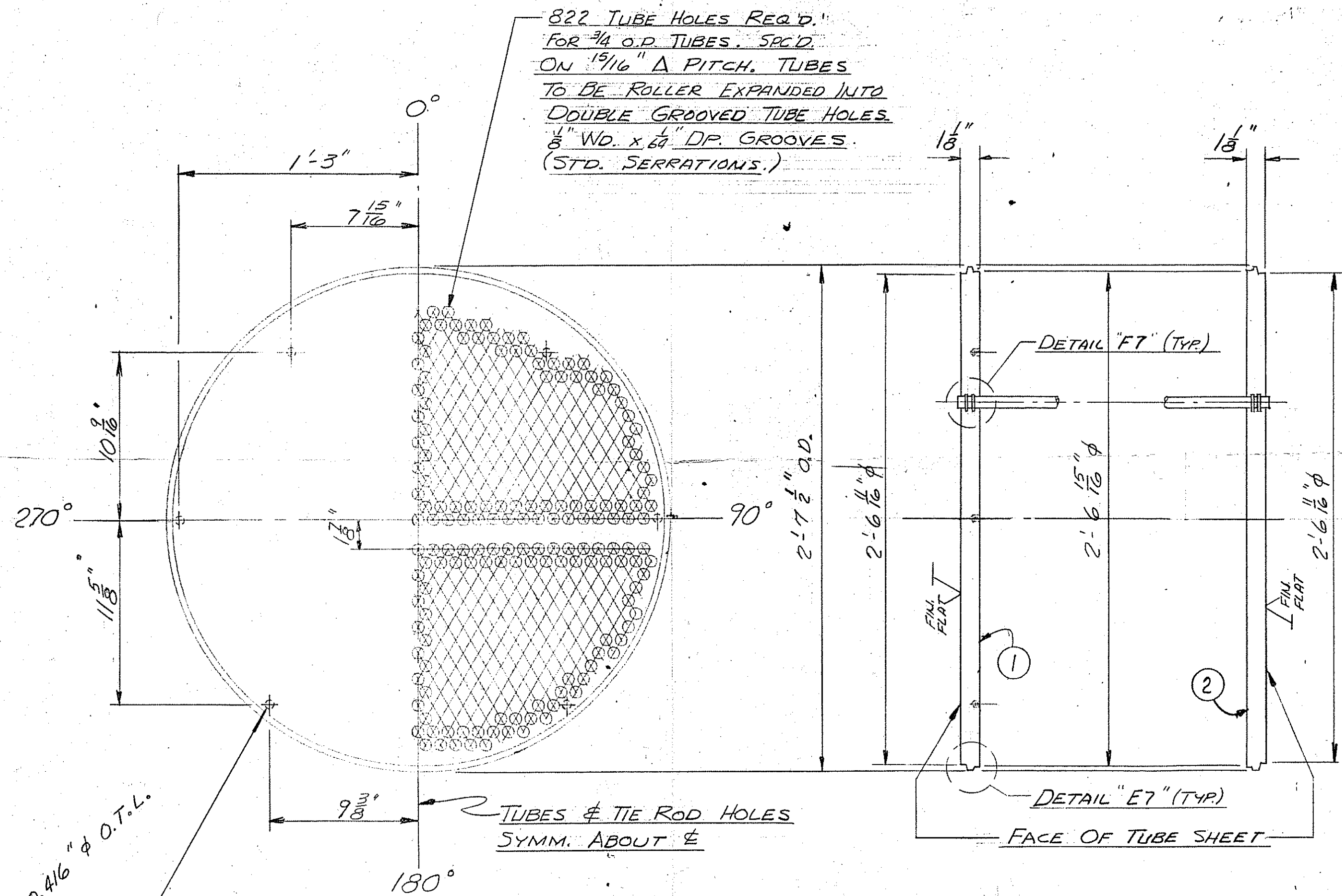
TUBE SHEET DETAIL ONE EACH REQ'D. MK. ① & ②
