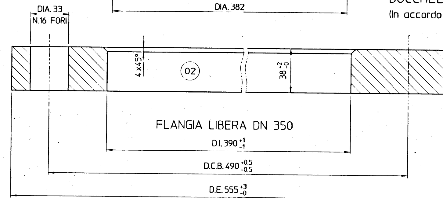
FLANGE DN 350 PN 25 UNI 2292-67 DM BOCCELLO MARCA 'F' (In accordo a std Montecatini F376)
