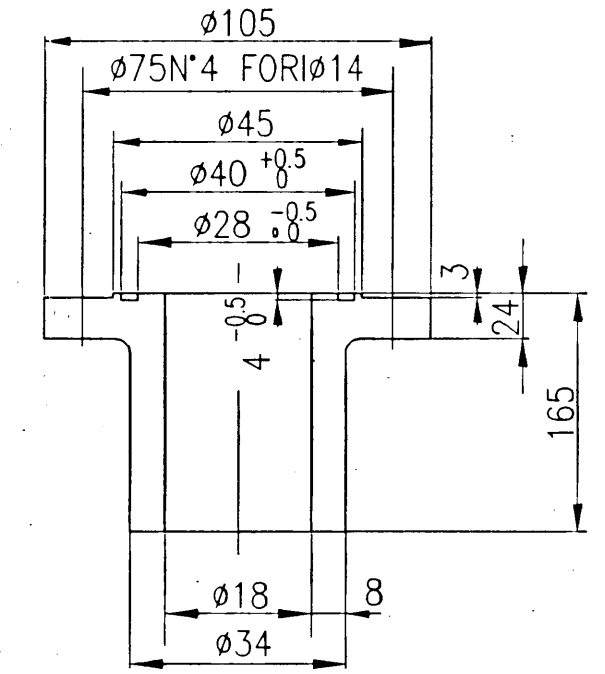
PART.FLANGIA LWN "AT" (113)
