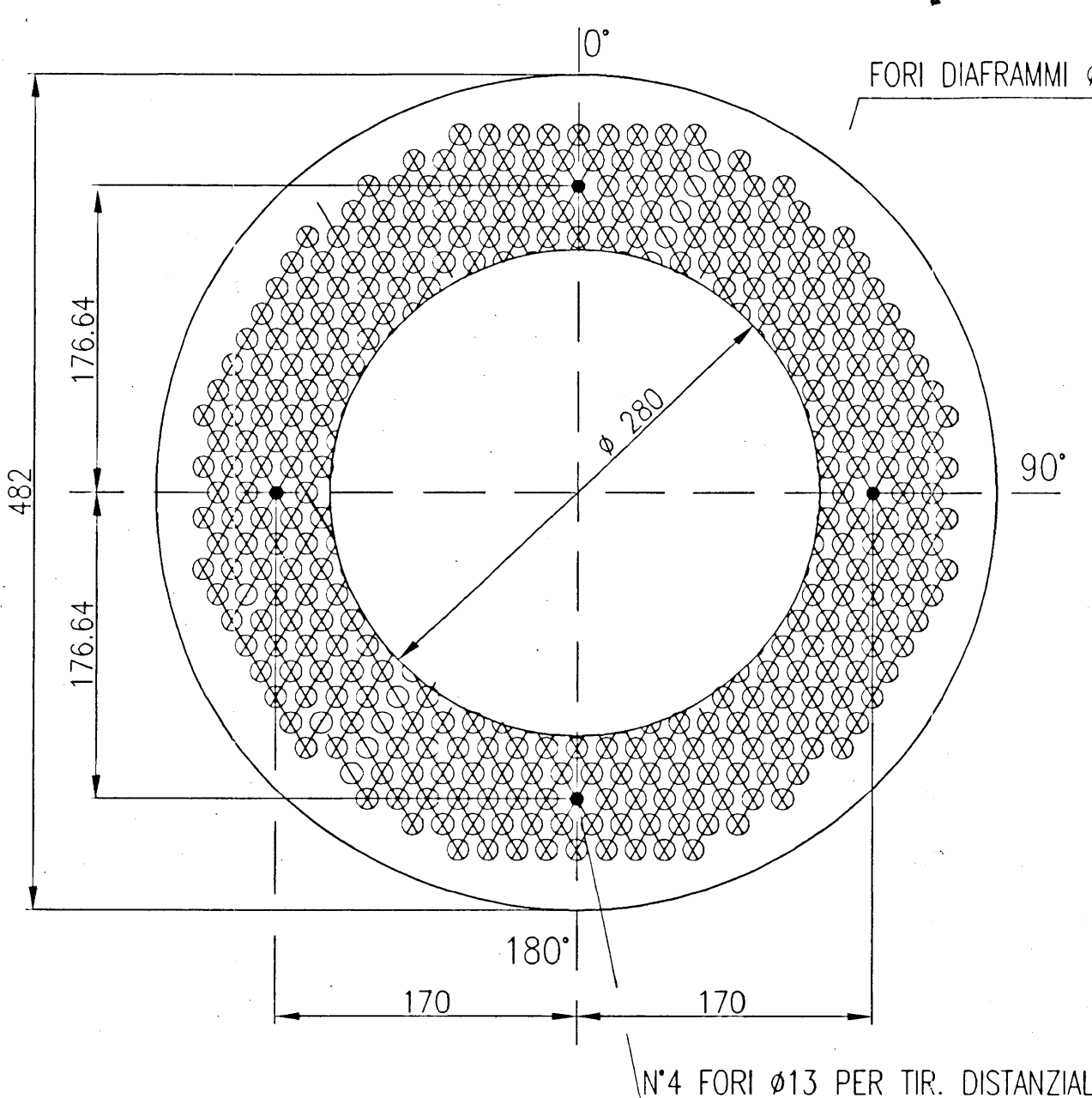
PART.FLANGIA LWN "AT" (113)
