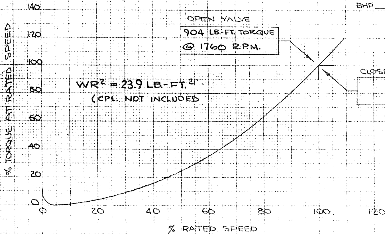
SPEED-TORQUE CURVE
