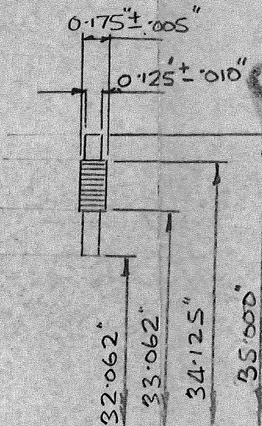
SECTION X-X
